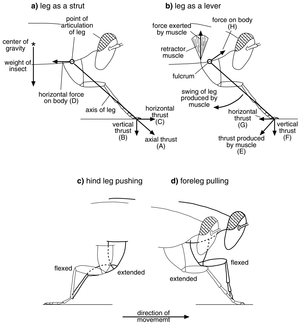
Fig. 8.12. Mechanical functioning of leg. (a) A leg acting as a strut. The axial thrust (A) is exerted down the length of the leg by virtue of the weight of the insect. The size of the axial thrust depends, among other things, on how much of the weight is borne by the other legs. It can be resolved into vertical and horizontal components (B and C), but because the foot is held by friction with the substratum it does not move. Instead, a horizontal force (D), equal and opposite to force (C) acts on the body and, in this case, tends to push it back unless balanced by other forces. (b) A leg acting as a lever. Contraction of the retractor muscle tends to swing the leg back so that the foot exerts a thrust (E) on the ground. This can be resolved into vertical and horizontal components (F and G), but since the foot is held still by friction an equal and opposite force (H) acts on the body pushing it forwards and upwards. (c) Extension of the coxotrochanteral and femoro-tibial joints of the hind leg pushes the body forwards. (d) Flexion of the coxotrochanteral and femoro-tibial joints of the foreleg pulls the body forwards.
