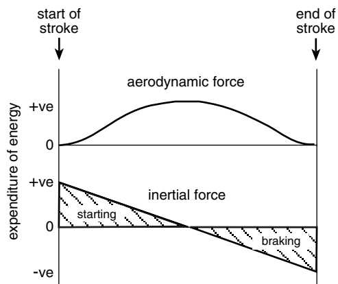
Fig. 10.20. The forces involved in moving a wing. At the start of the stroke, most energy is used overcoming the inertia of the wing. In midstroke, useful aerodynamic forces are produced. At the end of the stroke, the wing has considerable inertia (after Alexander, 1995).
