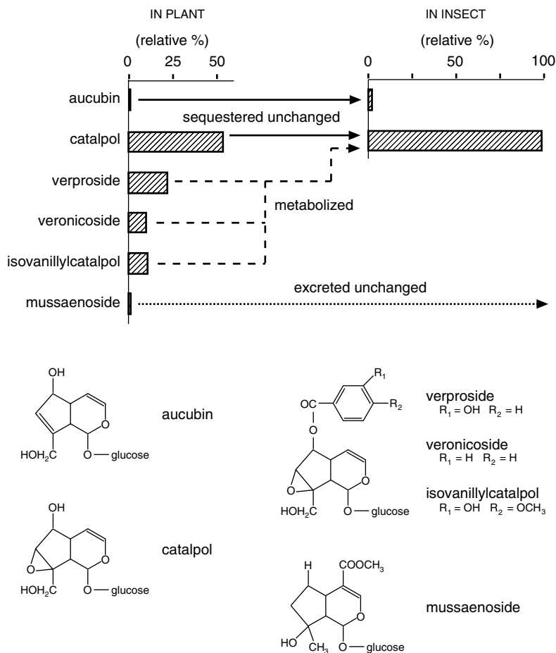
Fig. 27.20. Sequestration. Differential utilization of iridoid glycosides from a host plant, Besseyia plantaginea , by Euphydryas anicia . Aucubin and catalpol are sequestered unchanged, others are metabolized, and mussaenoside is not used. A proportion of all the compounds is excreted without being absorbed (based on Gardner & Stermitz, 1988; L'Empereur & Stermitz, 1990).
