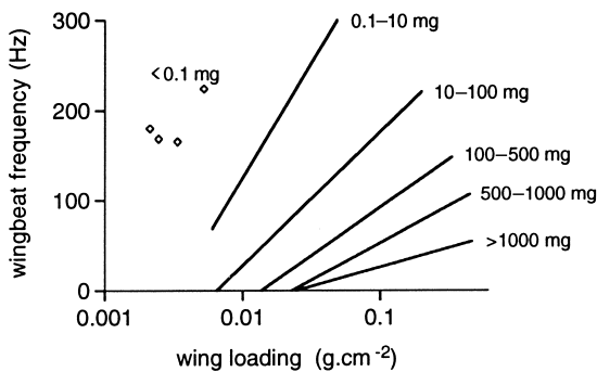
Fig. 9.22. Relationship between wing loading and wingbeat frequency for insects of different body weight. For insects weighing less than 0.1 mg, data are available for only four species, indicated by separate symbols (data from Byrne, Buchmann & Spangler, 1988).
