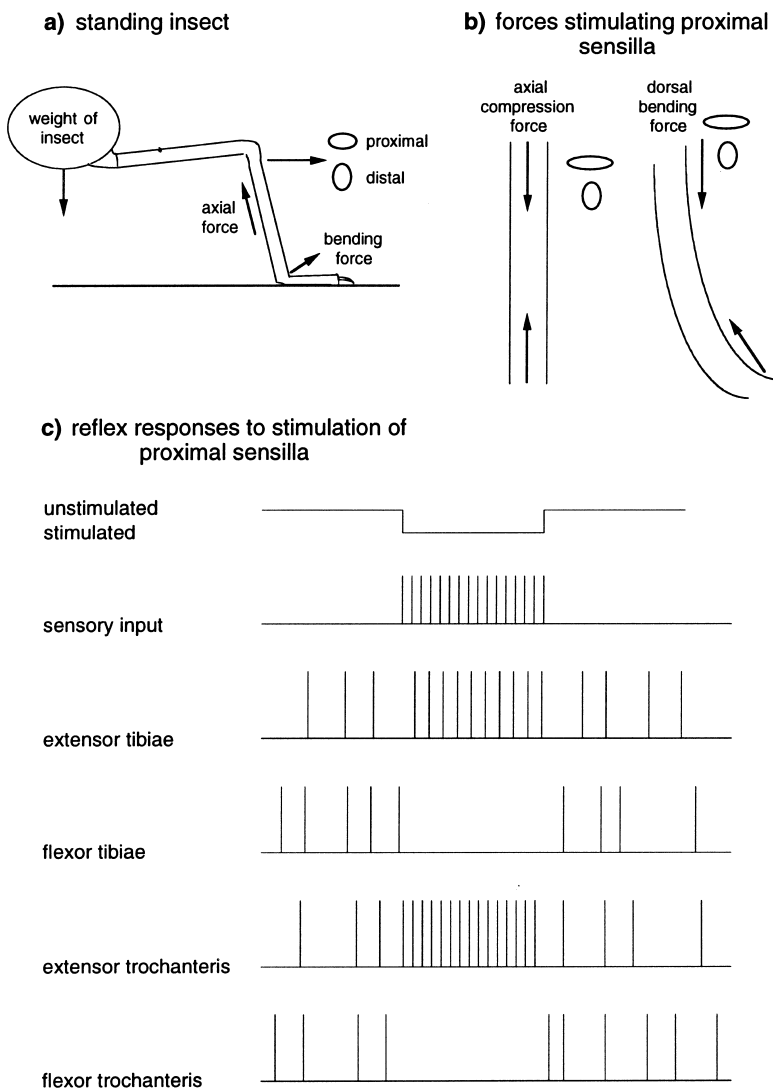
Fig. 8.11. Functioning of the proximal campaniform sensilla of a leg in a standing insect (based on Zill & Moran, 1981a; Zill et al. , 1981). (a) Cross-section of an insect. The two orientations of the sensilla in the proximal group are shown by the ellipses. (b) Diagram showing the effects of an axial force on dorsal bending. The transversely oriented sensilla, compressed along their short axes, are stimulated. (c) Activity in the motor neurons of tibial and trochanteral extensor muscles is enhanced when the sensilla are stimulated. The activity of the flexor muscles is inhibited. Vertical lines represent action potentials.
