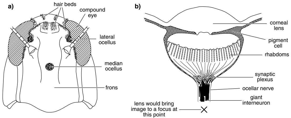
Fig. 22.20. Ocellus. (a) Frontal view of the head of a grasshopper showing the positions of the ocelli. (b) Diagrammatic longitudinal section through an ocellus of a grasshopper. The diagram shows the light-adapted condition with the pigment of the pigment cells restricting the entry of light. Notice that the image is focused below the rhabdoms (after Wilson, 1978).
