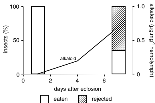
Fig. 27.23. Defence against predators. Relationship between alkaloid content of the hemolymph of adult beetles, Epilachna varivestis , and palatability to jumping spiders. By day 7 after eclosion, the beetles had a high concentration of alkaloid in the hemolymph and most were rejected by spiders (based on Eisner et al. , 1986).
