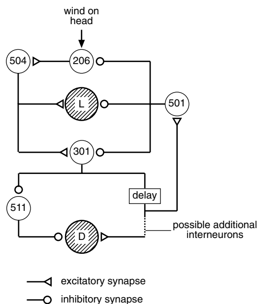
Fig. 20.25. Pattern generator. Diagrammatic representation of the interactions between a group of interneurons producing alternations in the contractions of the locust flight muscles. Interneurons represented by numbered circles; motor neurons hatched. L, motor neuron to levator muscle; D, motor neuron to depressor muscle (based on Robertson & Pearson, 1985).
