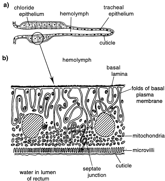
Fig. 3.14. Chloride cells in the rectum of a dragonfly larva. (Fig. 17.29 shows the position of the gills within the rectum). (a) Section of a rectal gill showing the position of the chloride epithelium. Note that tracheal epithelium refers to the epithelium of the gill through which gas exchange with the tracheae (not shown) occurs. (b) Details of the chloride cells. Notice that the luminal (water) side of the gill is at the bottom (after Schmitz and Komnick, 1976).
