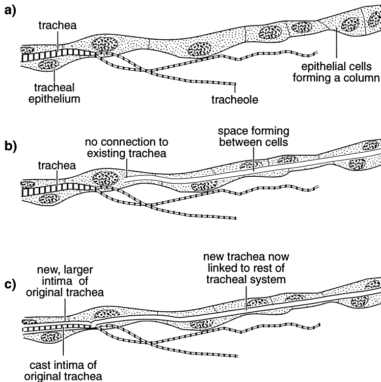
Fig. 17.7. Development of a new trachea as an extension of part of the existing system. Notice that the tracheolar cell is not shown (after Wigglesworth, 1954). (a) A column of cells extends from the tracheal epithelium. (b) A space develops between the cells of the column. (c) The space becomes lined by cuticle at a molt and connects with the new cuticle of the original trachea.
