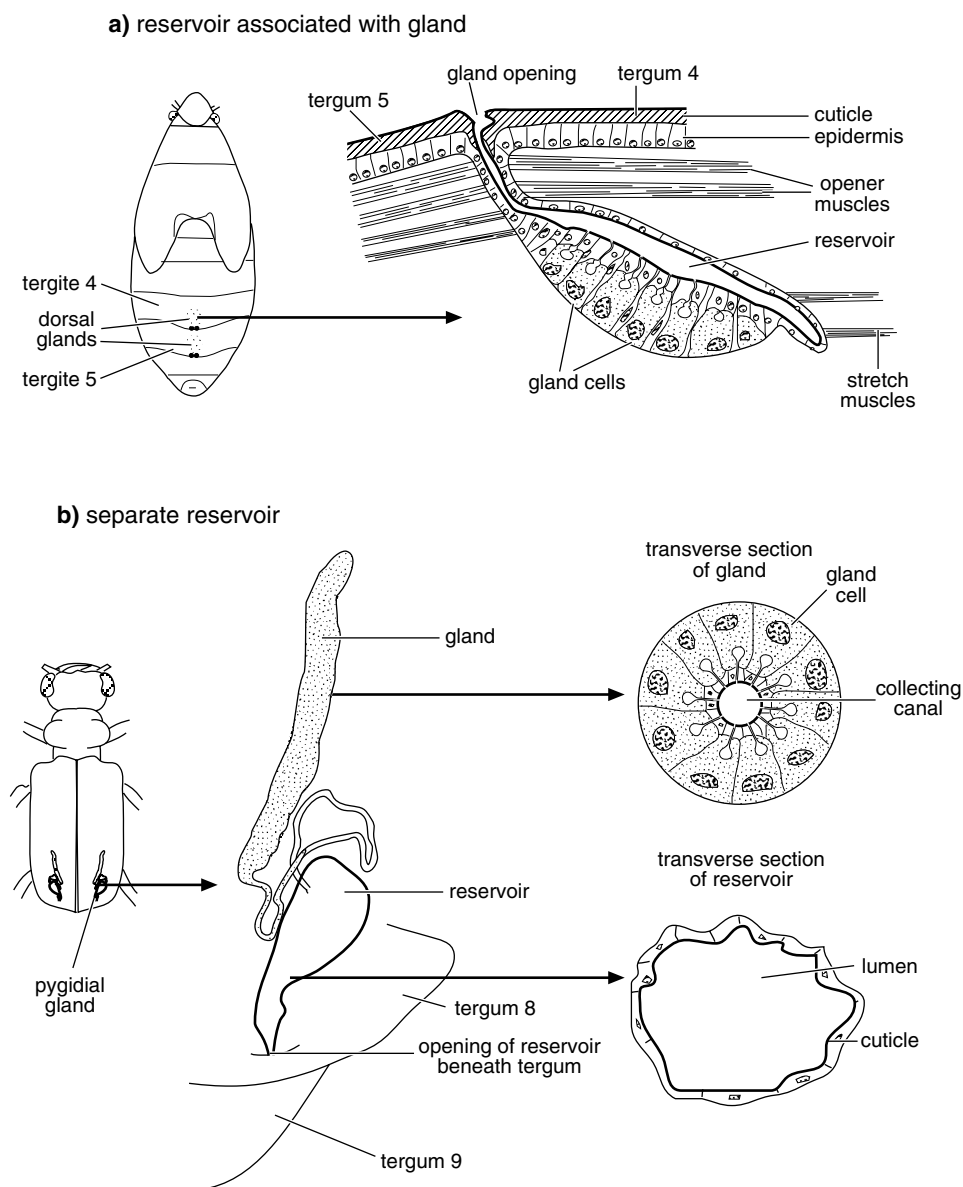
Fig. 27.16. Non-eversible exocrine glands. (a) Gland cells directly associated with reservoir. Abdominal glands of larval Heteroptera, Pyrhocris (after Staddon, 1979). (b) Gland cells separate from reservoir. Coleopteran pygidial gland, Cicindela (based on Forsyth, 1970).
