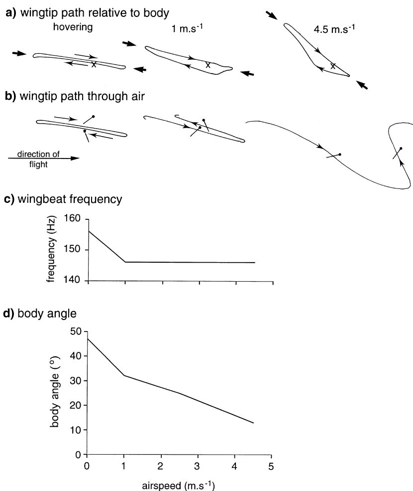
Fig. 9.20. Wingbeat of a bumblebee flying at different airspeeds (Hymenoptera, Bombus ) (after Dudley & Ellington, 1990a,b). (a) Path of the wingtip relative to the body (anterior to the right). Arrows at either end of the paths indicate the stroke plane. X shows the position of the wing base. (b) Path of the wing-tip as the insect flies from left to right. Short bars show the orientation of the wing at midpoints on the up and down strokes. The leading edge of the wing is indicated by a dot. (c) Wingbeat frequency. (d) Body angle. Notice that at high airspeeds the body angle decreases while the stroke plane angle (shown in a) increases.
