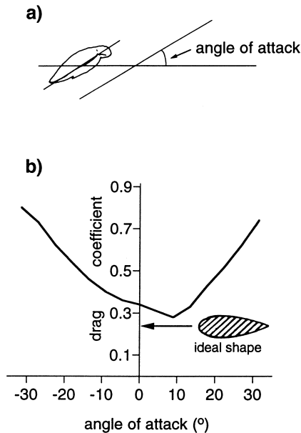
Fig. 8.31. Drag on a swimming beetle as its angle of attack changes (after Nachtigall, 1985).
