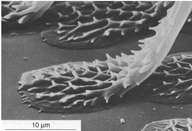
Fig. 8.8. Adhesive pads. (a) Tip of tenent hair of Philonthus (Coleoptera, Staphylinidae) (after Stork, 1983). (b) Suckers on the foreleg of male Dytiscus (Coleoptera, Dytiscidae) (after Miall, 1922).
