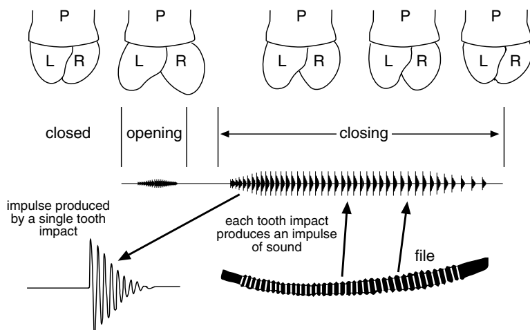
Fig. 26.5. Stridulation in bush crickets ( Ephippiger ). (a) Stridulatory mechanism. Top: opening and closing of the forewings (tegmina). In this species the wings are very short and not used for flying. P, pronotum; L, left tegmen; R, right tegmen. Center: the file showing how each tooth impact produces a sound impulse. Detail of a single impulse to the left (based on Pasquinelly & Busnel, 1955). (b) Frequency spectrum of the sound produced (based on Dumortier, 1963b).
