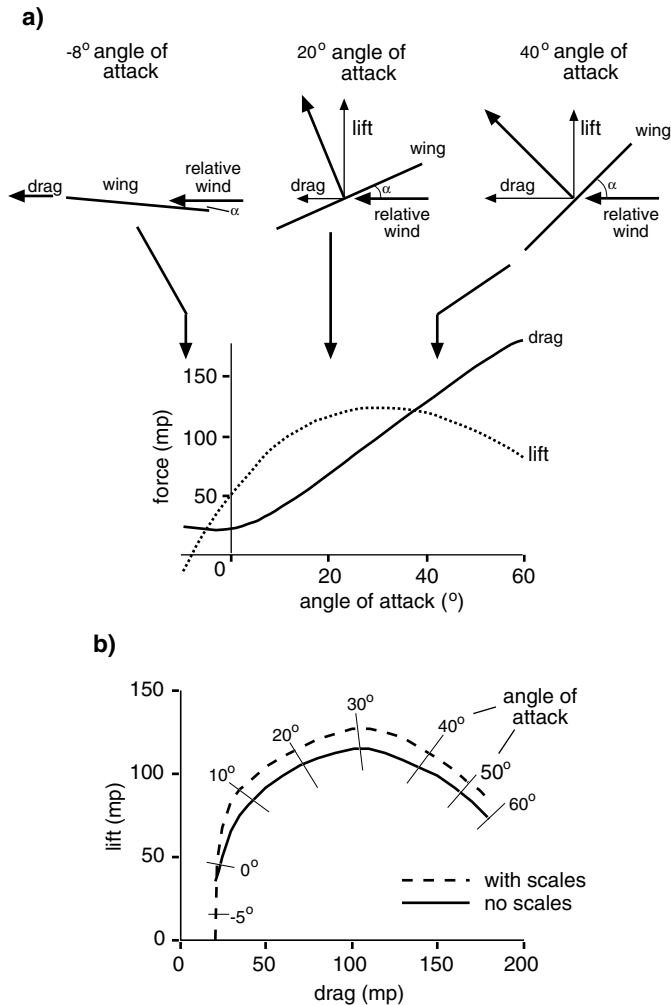
Fig. 9.30. Gliding. Experimental data from a moth which demonstrate the principles that would apply to any gliding insect (Lepidoptera, Agrotis ) (after Nachtigall, 1967). (a) Variations in lift and drag with the angle of attack. At the top are shown sections of the wing with various angles of attack ( \alpha ) corresponding to three points indicated by arrows on the graph. The insect is flying from left to right at a constant speed. (b) The relationship between lift and drag at different angles of attack showing the effect of removing the scales.
