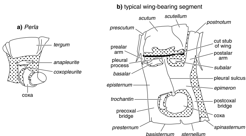
Fig. 7.5. Lateral view of thoracic segments. Anterior to left, membranous regions stippled. Names of sclerites in italics (after Snodgrass, 1935). (a) The prothorax of Perla (Plecoptera). (b) A typical wing-bearing segment.
