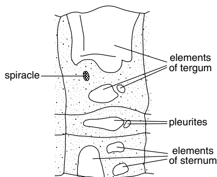
Fig. 11.3. Small sclerotized plates in an abdominal segment. Membrane stippled (larva of a beetle, Calosoma ) (after Snodgrass, 1935).
