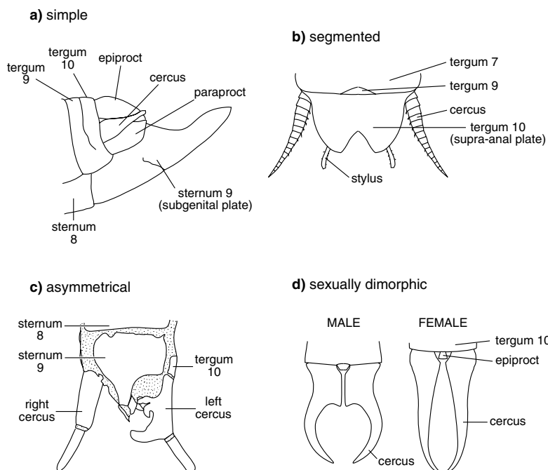
Fig. 11.7. Different types of cerci .
