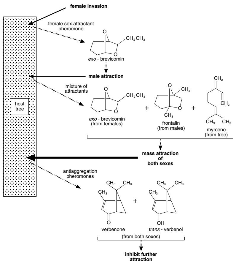
Fig. 27.12. Aggregation pheromones. Compounds involved in the invasion of a tree by the bark beetle, Ips paraconfusus .
