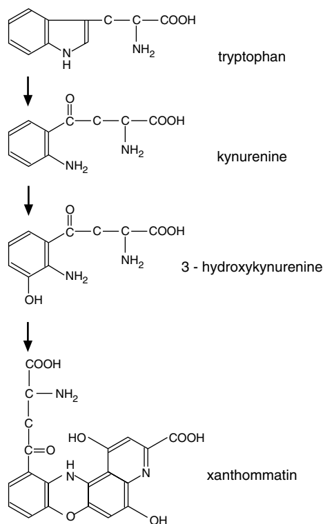
Fig. 25.6. Ommochromes. Synthesis of xanthommatin from tryptophan. Synthesis of other ommochromes involves the same pathway, differing in the final steps.
