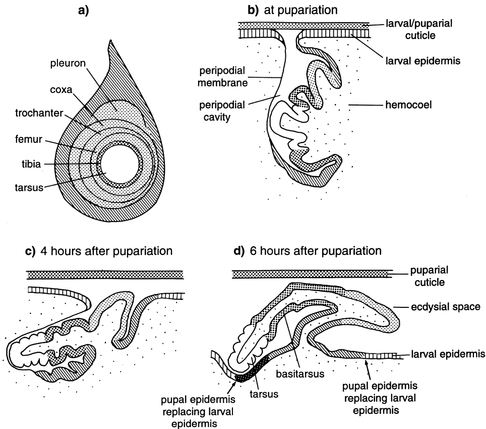
Fig. 15.20. Development of an adult leg in Drosophila . (a) Fate map of a leg disc (after Schubiger, 1971). (b)–(d) Sections through the disc at different times after pupariation showing the elongation and eversion of the leg (from Fristrom & Fristrom, 1993).
