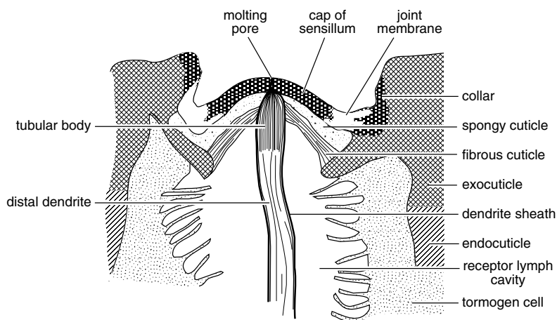
Fig. 23.2. Campaniform sensillum. Diagram showing the essential cuticular features. The arrangement of cells beneath the cuticle would be similar to that in Fig. 23.1.
