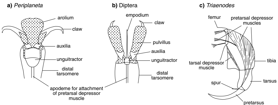
Fig. 8.4. Pretarsus. (a) Pretarsus of Periplaneta , ventral view (after Snodgrass, 1935). (b) Pretarsus of a dipteran, ventral view (after Snodgrass, 1935). (c) Distal part of prothoracic leg of larval Triaenodes (Trichoptera) showing a simple pretarsal segment (after Tindall, 1964).
