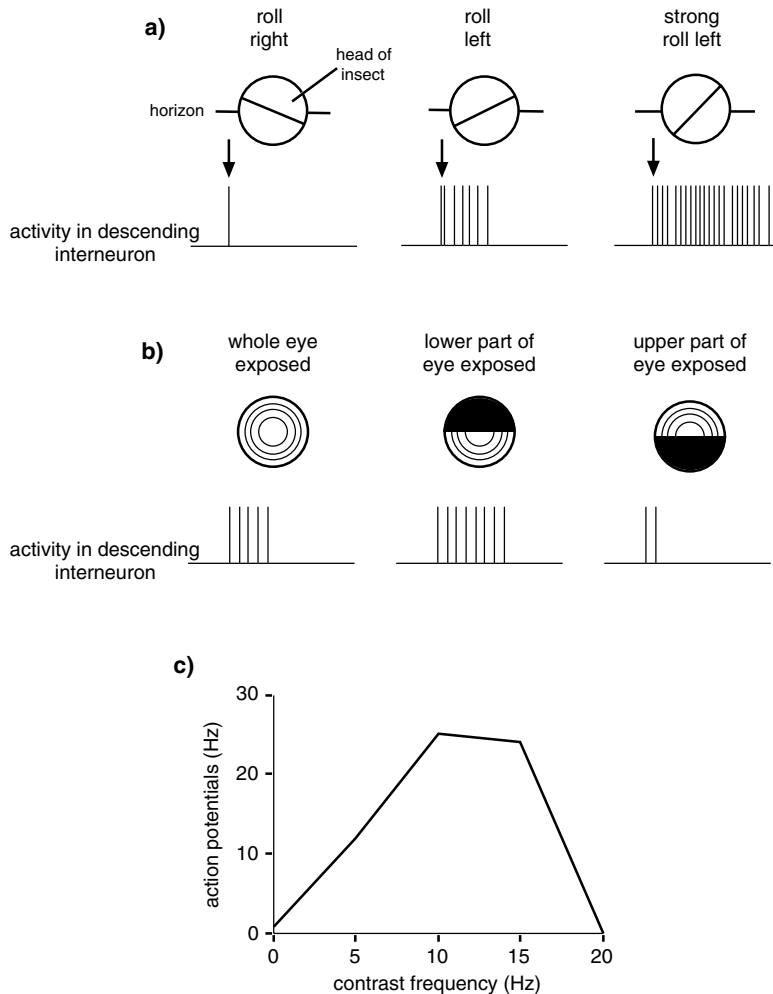
Fig. 9.34. Maintenance of stability. Examples of the activity of visually sensitive descending interneurons to perturbations of the visual field comparable with those occurring in flight in a locust ( Schistocerca ). (a) A wind-sensitive interneuron that responds to roll to the left. Arrows mark the onset of the wind (after Rowell & Reichert, 1985). (b) A neuron responding to image patterns simulating forward flight. The neuron responds most strongly when only the lower part of the eye is stimulated by the moving pattern, as would be the case in normal flight. Interneurons with these characteristics are probably involved in the optomotor response (based on Baader et al. , 1992). (c) The sensitivity of a neuron similar to that in (b) to different rates of pattern movement (contrast frequency) over the eye (data from Baader et al. , 1992).
