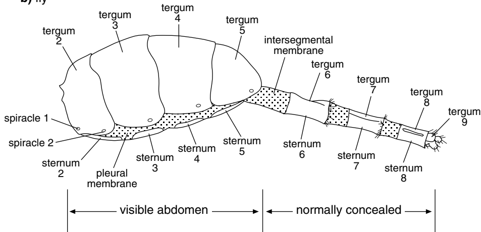
Fig. 11.1. Abdomen in lateral view. (a) An insect in which parts of all 11 segments are present in the adult (female red locust, Nomadacris (Orthoptera)) (after Albrecht, 1956). (b) An insect with a reduced number of segments in the adult. Segments 6–9, which form the ovipositor, are normally retracted within the anterior segments (female housefly, Musca (Diptera)) (after Hewitt, 1914).
