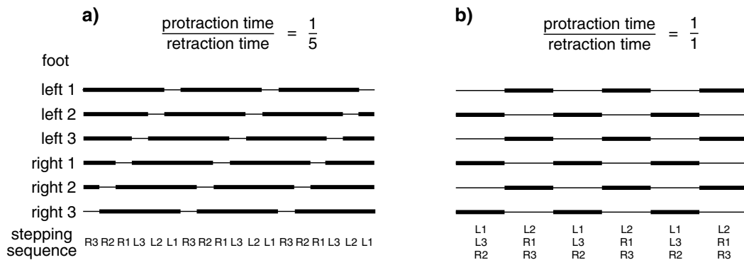
Fig. 8.14. Stepping patterns. Diagram showing the disposition of the feet with different protraction time:retraction time ratios. Thick lines indicate retraction with the foot on the ground, thin lines protraction with the foot in the air (based on Hughes, 1952)
