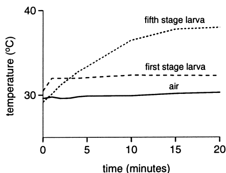
Fig. 19.4. Effect of solar radiation on body temperature of a locust ( Schistocerca ). At time 0, the insects were placed in the sun, having previously been in shade. The larger, fifth stage larva reaches a higher temperature but heats up more slowly than the smaller first stage larva (after Stower & Griffiths, 1966).
