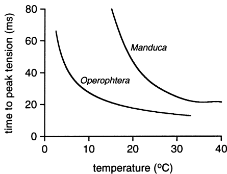
Fig. 19.11. Flight at low temperatures. The time for the flight muscles to reach peak tension is shorter in the winter moth, Operophtera , which flies at low thoracic temperatures, than in Manduca which only flies when the thoracic temperature is above 30°C (after Marden, 1995).
