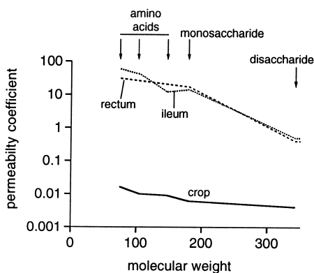
Fig. 3.13. Permeability of the intima of the fore and hindgut of Schistocerca . Notice that the permeability coefficient is shown with a logarithmic scale. Arrows at the top show the molecular weights of some of the compounds in the gut (based on Maddrell & Gardiner, 1980).
