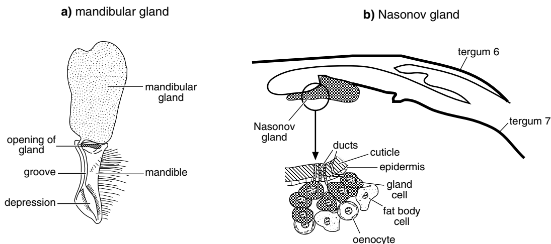
Fig. 27.3. Two exocrine glands of worker honeybees: (a) mandibular gland and mandible (after Snodgrass, 1956); (b) Nasonov gland, with part of the gland enlarged (below).
