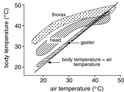
Fig. 19.9. Thermoregulation in the honeybee ( Apis ). Each shaded area represents the range of temperatures recorded from bees in free flight. Notice that at higher air temperatures, head and thoracic temperatures rise less sharply than at lower temperatures. This results from the cooling effects of evaporative water loss from nectar droplets on the mouthparts. The temperature of the gaster is always close to air temperature (body temperature = air temperature). It plays no part in cooling. (Compare Fig. 19.3c) (after Heinrich, 1980a,b).
