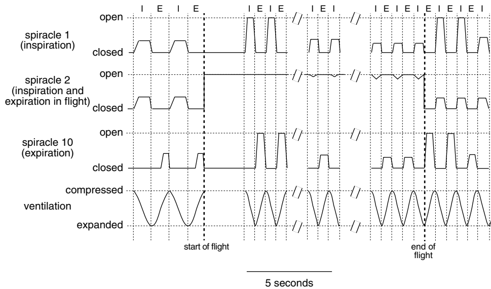
Fig. 17.20. Spiracle activity and abdominal ventilation during flight of Schistocerca . I, inspiration; E, expiration (after Miller, 1960c).
