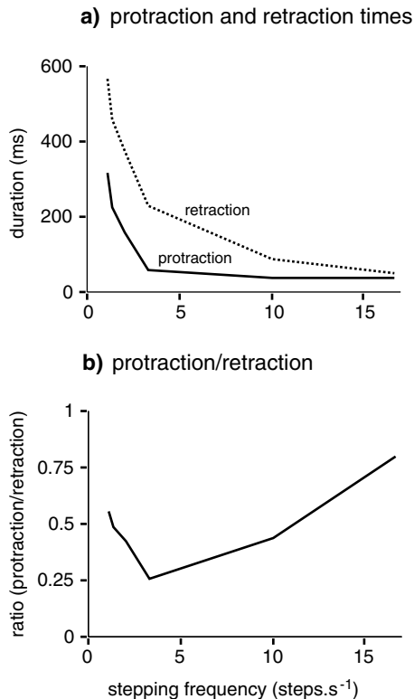
Fig. 8.17. Mechanics of locomotion. Changes in duration of retraction and protraction times of a leg in Periplaneta in relation to the stepping frequency (after Delcomyn & Usherwood, 1973). (a) Protraction and retraction times. (b) Ratio of protraction/retraction.
