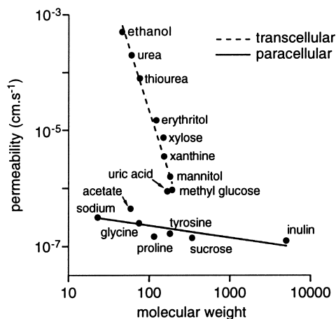
Fig. 18.6. Production of primary urine. Passive movement of solutes into the unstimulated Malpighian tubules of Rhodnius . Charged substances, such as sodium, glycine and tyrosine, as well as larger molecules, move between the cells (paracellularly). (Note that sodium is actively transported through the cells when the Malpighian tubules are stimulated by diuretic hormone.) Uncharged substances, such as urea and mannitol, move much more quickly although they have similar molecular weights to glycine and tyrosine. They probably diffuse through the cells (transcellularly) (based on O'Donnell & Maddrell, 1983).
