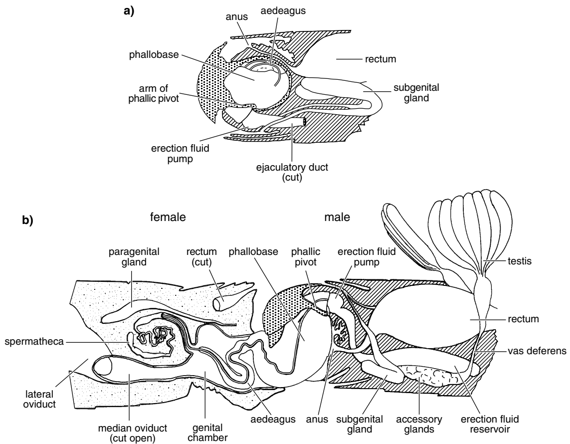
Fig. 12.10. Male genitalia and direct insemination ( Oncopeltus , Hemiptera) (after Bonhag & Wick, 1953). (a) Sagittal section of the male genital capsule with the aedeagus retracted. (b) Sagittal section through the terminal segments of a copulating pair. Notice the inversion of the male genital capsule (with the anus now ventral to the phallic pivot) and the insertion of the aedeagus into the spermatheca.
