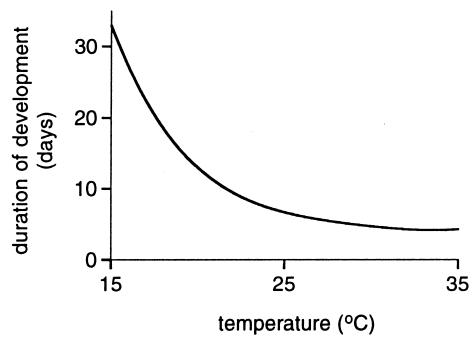
Fig. 14.28. The effect of temperature on the duration of embryonic development (milkweed bug, Oncopeltus , Hemiptera) (from Richards, 1957).
