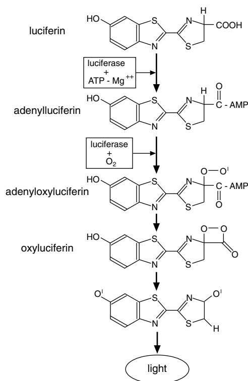
Fig. 25.17. Basic reactions involved in light production from luciferin.
