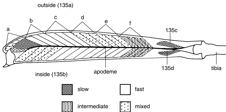
Fig. 10.4. Arrangement of fibers with different properties in the extensor tibiae muscle of a locust. Shading shows the dominant type of fiber in each region. Lettering indicates the type of innervation (see Table 10.1) and numbers indicate the anatomically distinct parts of the muscle (after Hoyle, 1978b).
