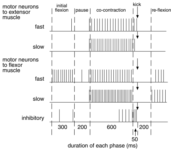
Fig. 8.24. Jumping. Activity of the motor neurons controlling the extensor and flexor tibiae muscles of the hind leg of a locust in relation to a jump. Vertical lines represent action potentials (after Heitler & Burrows, 1977).
