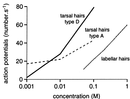
Fig. 24.10. Differences in threshold of sucrose-sensitive neurons in different sensilla of the blowfly (data from McCutchan, 1969; Omand & Dethier, 1969).
