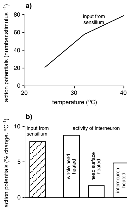
Fig. 19.18. Effect of temperature on mechanosensory input from the wind-sensitive hairs on the head and the activity of a giant interneuron in the brain of a grasshopper, Schistocerca americana (after Miles, 1992). (a) Sensory input (action potentials per stimulus) from a single hair deflected by 29 \mu\text{m} at different temperatures. (b) Changes in responses, expressed as percentage change in the frequency of action potentials for each ^{\circ}\text{C} change in temperature. Input from the wind-sensitive hairs increased sharply when they were heated, but the central response, as indicated by the activity of the interneuron, was dependent on the temperatures of both the sensory cells and of the interneuron. If both experienced a rise in temperature (whole head heated), the interneuron responded sharply to a change in temperature; if only the temperature of the mechanoreceptors was affected (head surface heated), the interneuron showed little change in activity; if the temperature of the interneuron increased, but that of the sensory neurons did not (interneuron heated) its activity increased, but to a lesser extent than if the whole head was heated.
